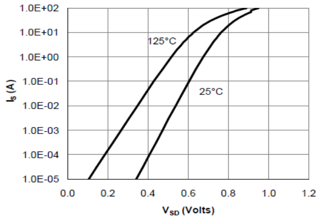
Figure 6: Body-Diode Characteristics
