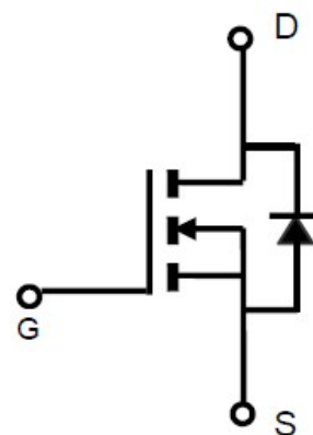
N-Channel
