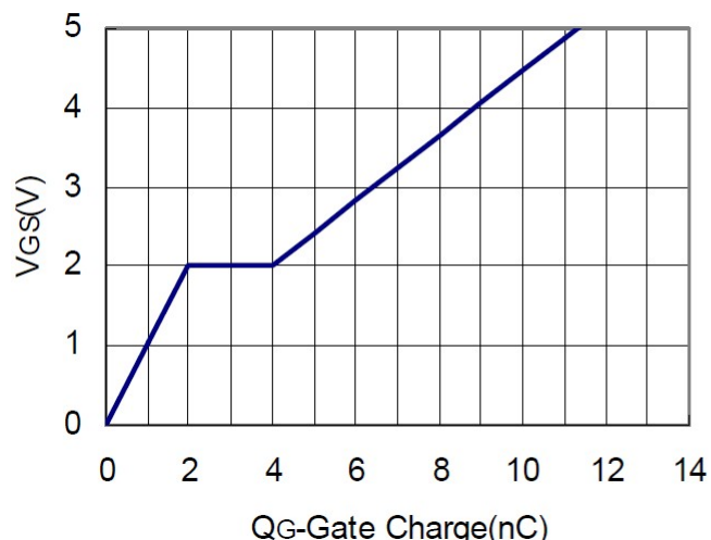
Gate Charge
